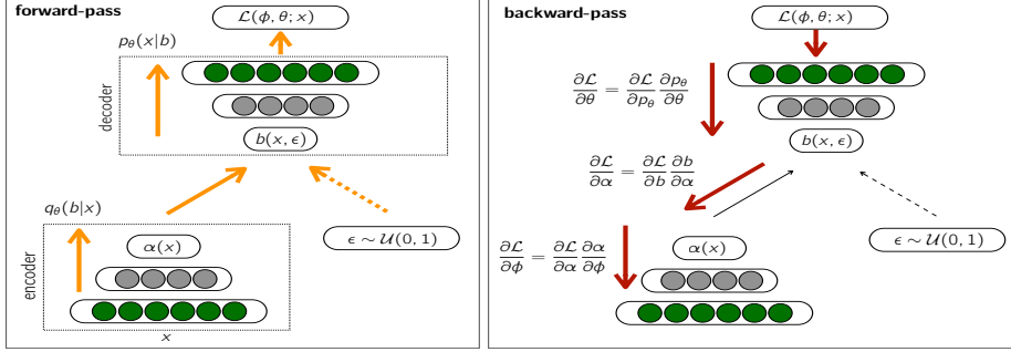
Fig. 2. Illustration of the forward (orange) and backward (red) pass implementing the proposed method as a deep neural net. The dashed line represents a stochastic layer.
