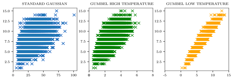
Fig. 4. Similarity before tresholding ( x -axis) and after tresholding ( y -axis) for 10^5 pairs of samples drawn from different latent distributions (32-bits).
