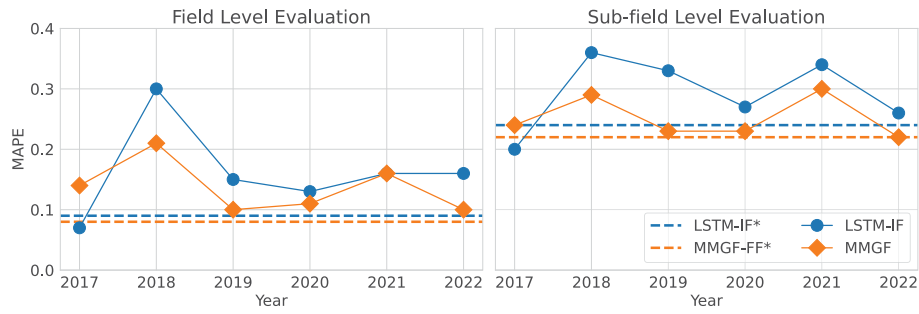
Fig. A.12. Results at different years. MAPE of the crop yield prediction across years in the leave-one-year-out evaluation for ARG-S fields. *As a comparison, the dashed lines show the model performance in the stratified 10-fold cross-validation. The LSTM-IF uses S2-M with DEM modalities, while the MMGF use all modalities (S2-R, weather, DEM, soil). There are 8, 12, 19, 50, 73, and 27 (validation) fields respectively for each year from 2017 to 2022.
