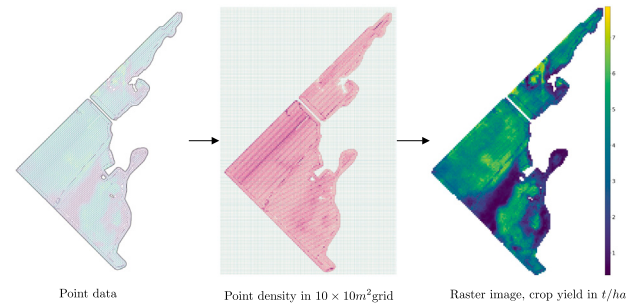
Fig. 1. The figure depicts the rasterization process for the ground truth yield data, where a cleaned point vector data (left) for a field is aligned with the satellite image, and the mean of all yield points within one pixel is assigned to that pixel. The resulting raster image is referred to as the yield map in this study.
