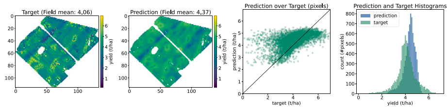
(b) Predictions of MMGF model with S2-R, weather, DEM, and soil modalities as input.
